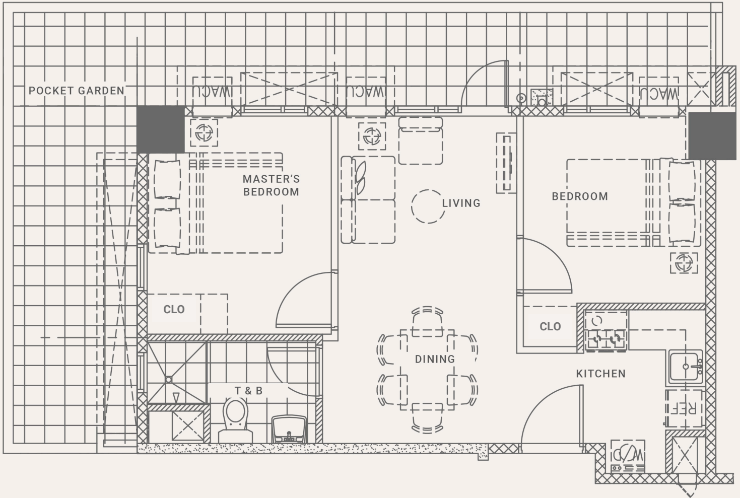
UNITS J & S Unit Area: ± 72.5 sq.m
